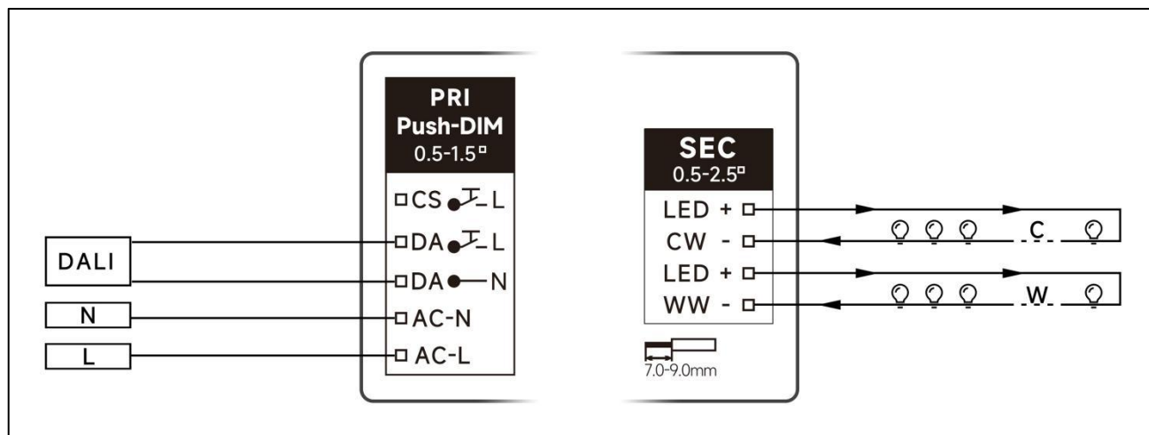
DALI Connection
